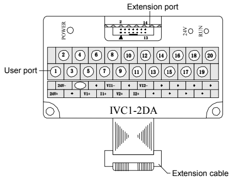
Figure 1-2 IVC1-2DA ports
