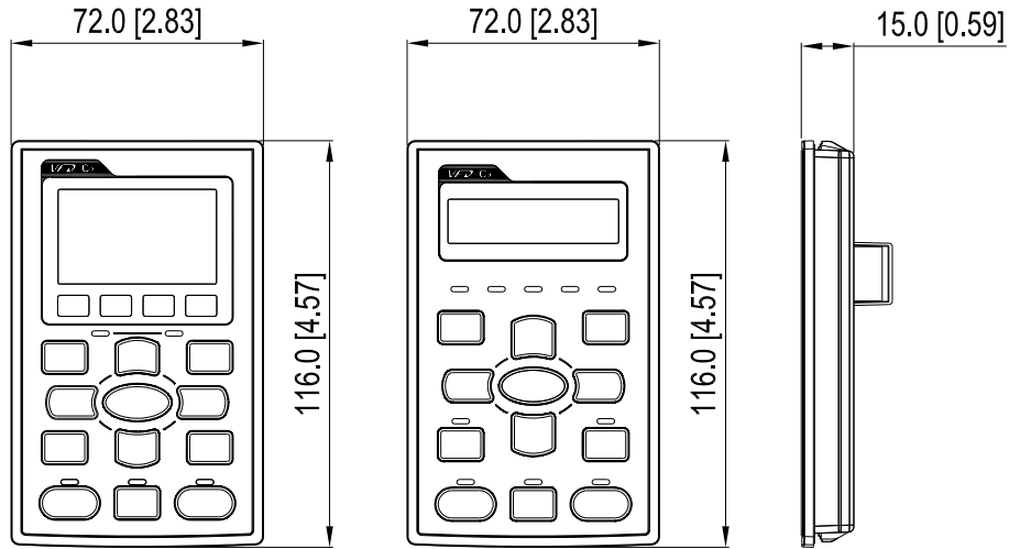
KPC-CC01 Standard LCD Keypad KPC-CE01 Optional LED Keypad
